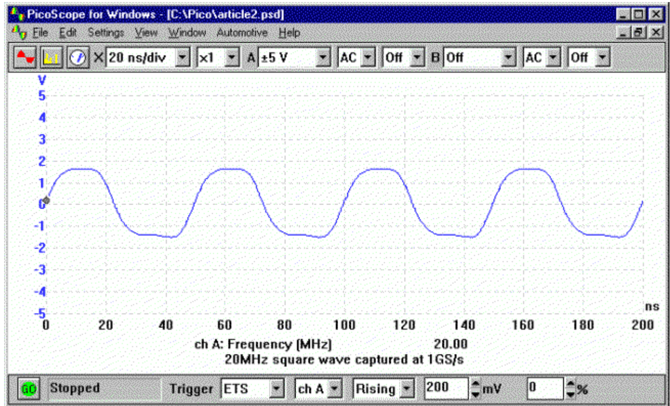
Figure 1b: 20MHz square wave captured at 1GS/s.
