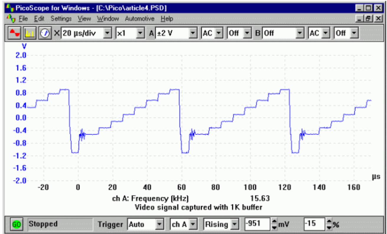
Figure 2a: 200 \mu\text{s} of a video wave captured with a 1 K buffer memory.
